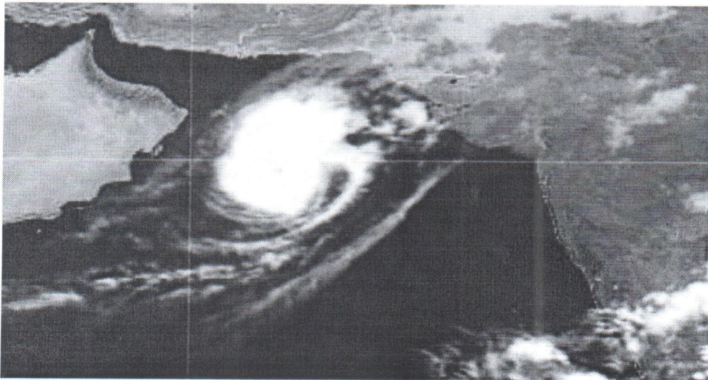
IR Satellite imagery at 1000 PST, 29 October 2019
